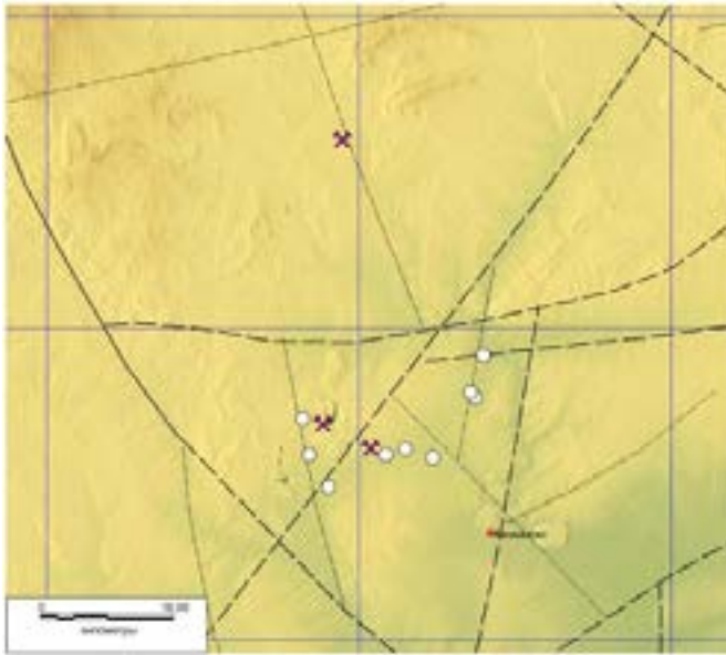
— — — faults; ○ – epicenter; – open pit. Fig. 2. The Zhezkazgan earthquake epicenter
